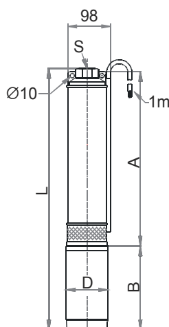
Pump Units C-SJ5-8, C-SJ8-5
